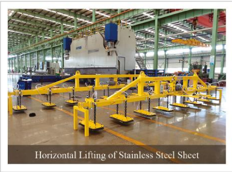
AC-Vacuum Lifter (8 Suckers) HP-BLJ8000-8S (8000KG)
