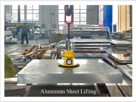
Mechanical Vacuum Lifter (Single Sucker) HP-WDL80-1S (80KG)
