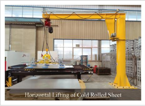
AC-Vacuum Lifter (6 Suckers) HP-BSJ1000-6S (1000KG)
