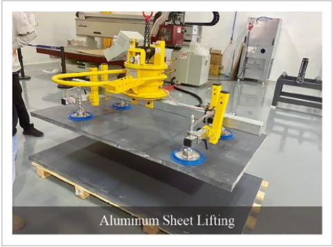
Mechanical Vacuum Lifter (4 Suckers) HP-WDL800-4S (800KG)
