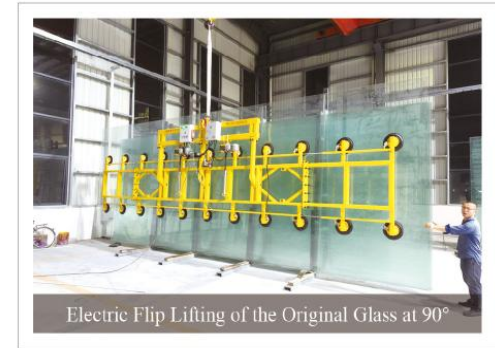
AC -Vacuum Lifter (22 Suckers) HP-DF2000-22S (2000KG)
